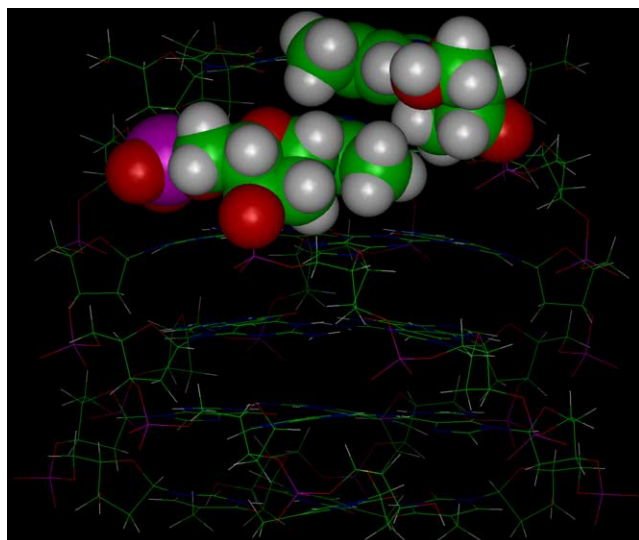
Figure 5. Side view of average structure of the best 10 structures of II . Heavy atoms are shown with different colors (carbons, green; nitrogens, blue; oxygens, red; hydrogens, white). One A^{8Me} residue and the dT residue of the same strand are reported in CPK. Steric effect between methyl of A^{8Me} and the dT residue is plainly observable.
