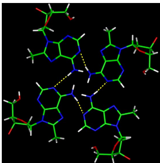
Figure 4. A 8Me -tetrad observed in the mean structure of I . Heavy atoms are depicted in colored 'stick' (carbons, green; nitrogens, blue; oxygens, red; hydrogens, white). Dashed yellow lines represent hydrogen bonds.
