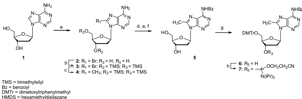
Scheme 1. Synthesis of phosphoramidite derivative 7 . Reagents and conditions: (a) Br 2 in acetate buffer; (b) hexamethyldisilazane, (NH 4 ) 2 SO 4 in dry dioxane; (c) Pd(PPh) 4 , (CH 3 ) 4 Sn in N -methylpyrrolidinone; (d) trimethylsilyl chloride in dry pyridine; (e) benzoyl chloride in dry pyridine; (f) H 2 O/NH 3 ; (g) dimethoxytriphenylmethyl chloride in dry pyridine; (h) 2-cyanoethyl-N,N-diisopropyl chlorophosphoramidite in dry CH 2 Cl 2 .
