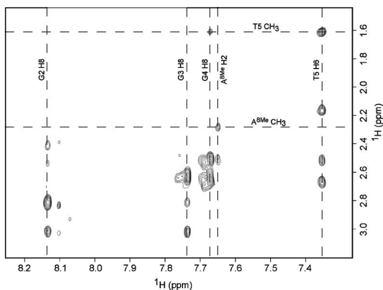
Figure 2. Expanded region of a NOESY spectrum (500 MHz, 180 ms mixing time, T = 30 °C) containing aromatic and H2′/H2″ sequential crosspeaks and NOEs involving methyl groups of I .
