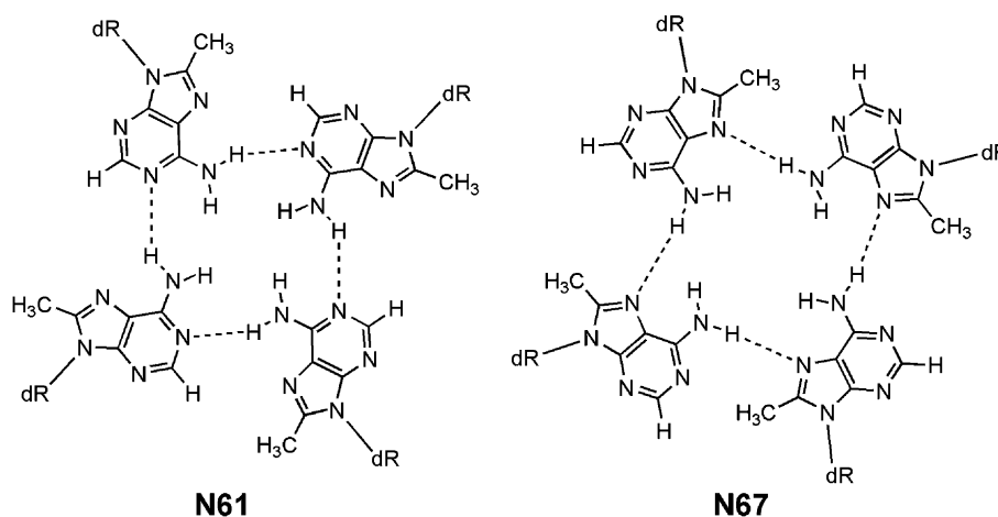
Figure 3. N61 and N67 H-bond patterns for an A-tetrad. H-bonds are indicated by dashed lines.
